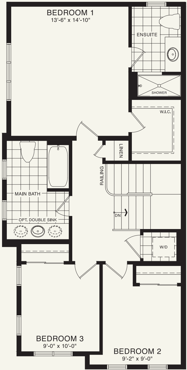
SECOND FLOOR PLAN STYLE A1
