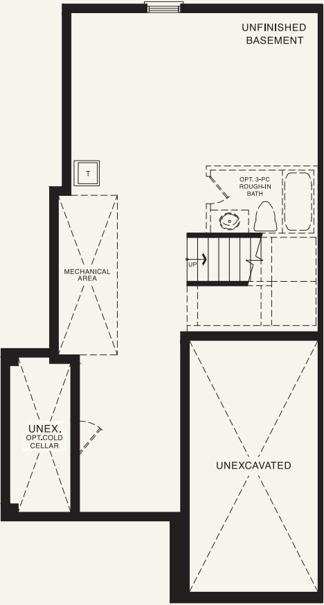
BASEMENT PLAN STYLE A1
